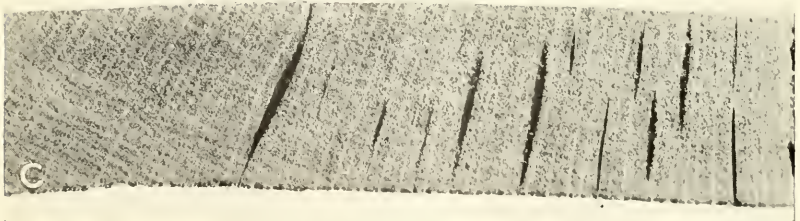
A surface check in a 6/4-inch hardwood board closed by compression of the surface fibers during the latter part of the seasoning period: A, Normal appearance of the surface; B, the sides of the check forced apart at one surface; C, cross section of the board at the check
